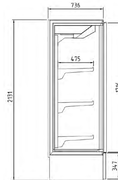
Detalle estante inclinado Inclined shelf detail
