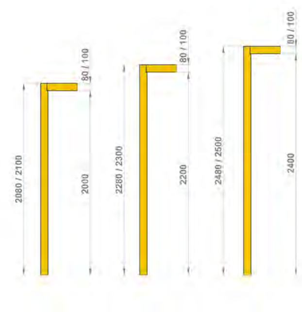
SIN suelo panel WITHOUT floor panel
