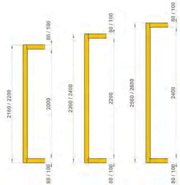
CON suelo panel WITH floor panel
