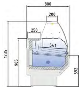
Vitrinas NO MODULARES - PLUG &amp; PLAY units, not modular
