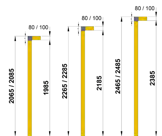
SIN suelo panel WITHOUT floor panel
