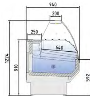
Vitrinas NO MODULARES - PLUG &amp; PLAY units, not modular
