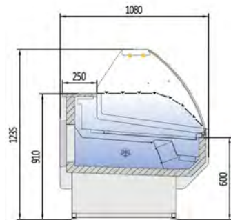
Vitrinas NO MODULARES - PLUG &amp; PLAY units, not modular
