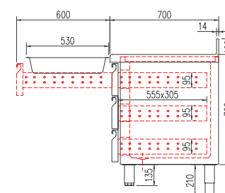
MRG-200 con cajones auto-cierre y ruedas with soft-closing drawers and castors
