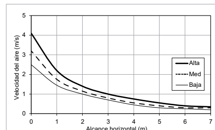
MMK-UP0151HP(L)-E
