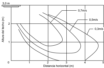
MMU-UP0481HP-E, UP0561HP-E
